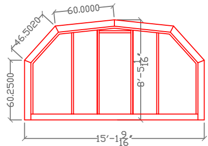
13' Enclosure bay 3
