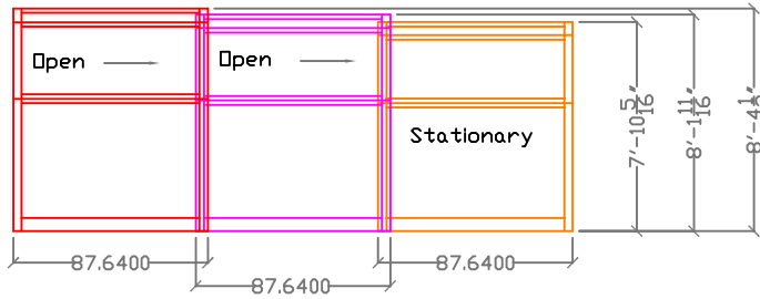
Side Elevation
