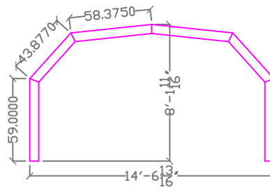
13' Enclosure bay 2
