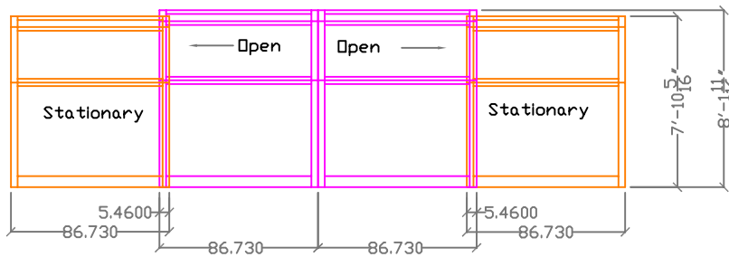
Side Elevation
