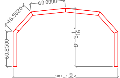
13' Enclosure bay 3
