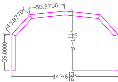
13' Enclosure bay 2
