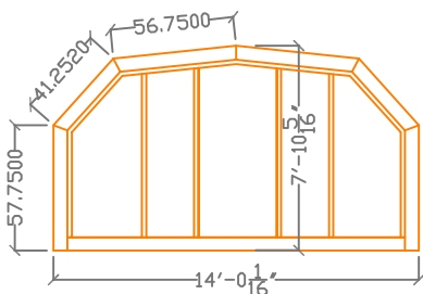
13' Enclosure bay 1
