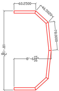
16' Enclosure bay 3
