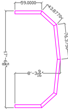
16' Enclosure bay 2
