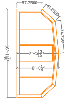
16' Enclosure bay 1
