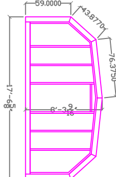
16' Enclosure bay 2
