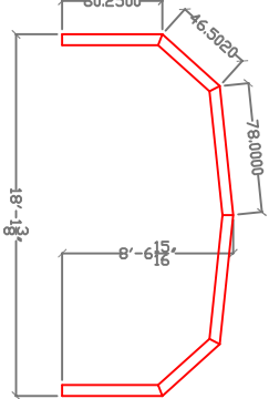
16' Enclosure bay 3
