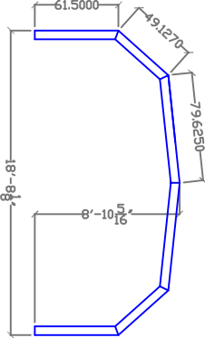
16' Enclosure bay 4
