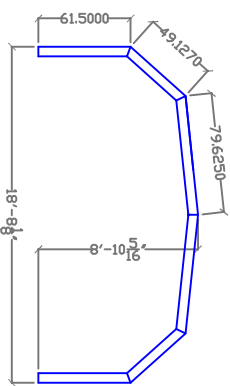
16' Enclosure bay 4
