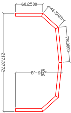
16' Enclosure bay 3
