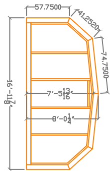
16' Enclosure bay 1
