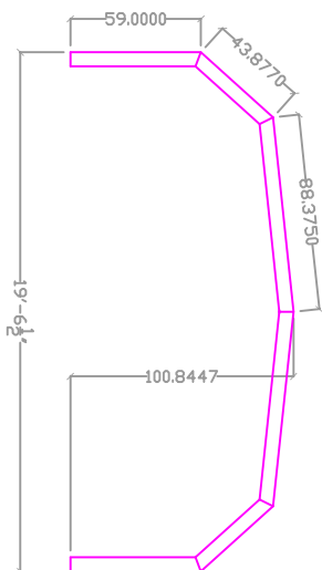
18' Enclosure bay 2
