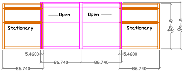
Side Elevation
