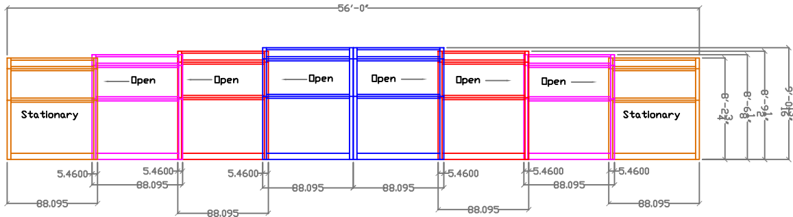
Side Elevation
