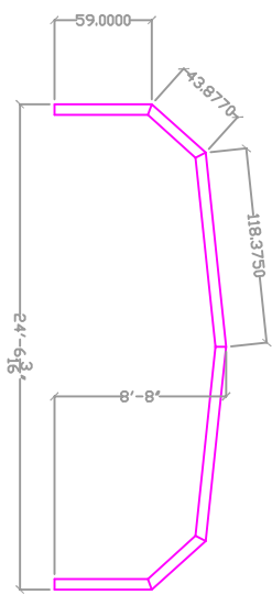
23' Enclosure bay 3
