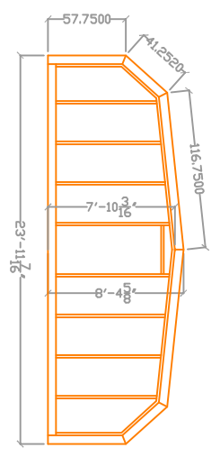
23' Enclosure bay 2
