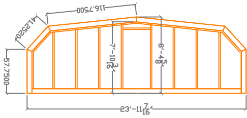
23' Enclosure bay 1
