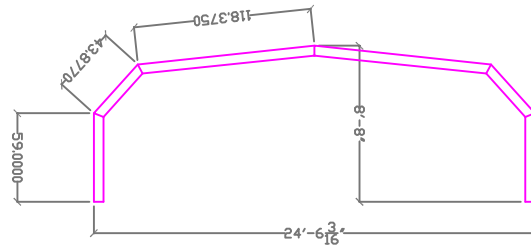
23' Enclosure bay 2
