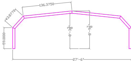
26' Enclosure Bay 2
