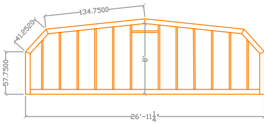
26' Enclosure bay 3
